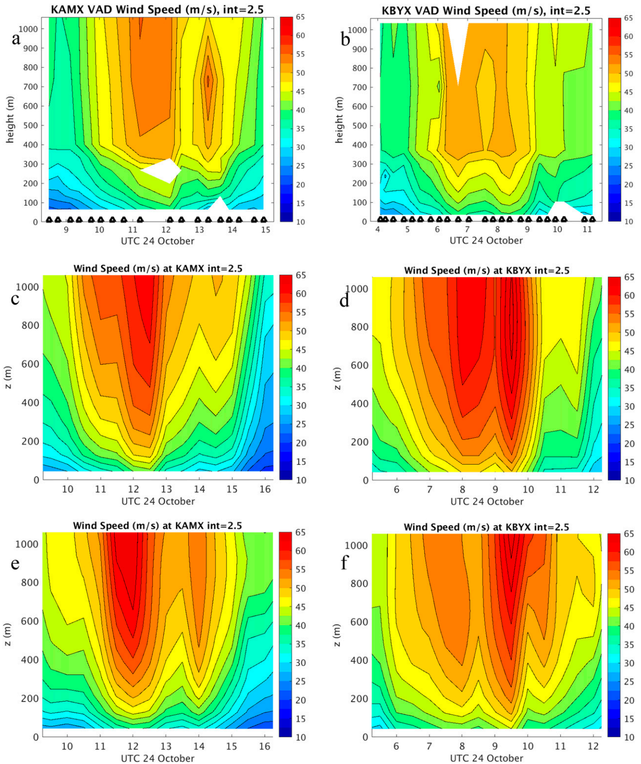
FIG. 11. Time–height profiles of wind speed at the Miami and Key West radar stations: (a) VAD profiles at KAMX; (b) VAD profiles at KBYX; (c) FinalYSU at KAMX; (d) FinalYSU at KBYX; (e) FinalMYJ at KAMX; (f) FinalMYJ at KBYX. Note that the time range is shifted 1 h later for the simulations. The analysis times for each VAD profile are indicated by the black triangles. The model data were computed on the hour and half hour.
